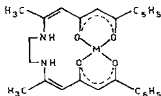
ISOMER II
