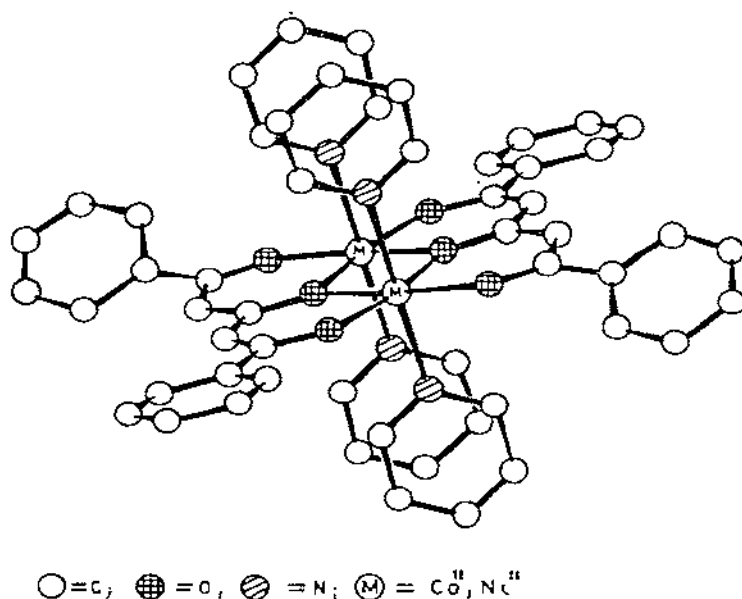
Fig. 16. Molecular structure of the complexes bis-(1,5-diphenyl-1,3,5-pentanetrionato)-tetrapyridinedicobalt(II) or dinickel(II).
