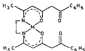
ISOMER I
