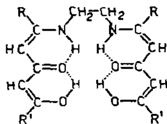
Fig. 20. The prepared open sexadentate ligands ( R=CH_3 ; R' = substituted phenyl group).
