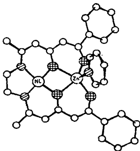
Fig. 22. A view of the molecular structure of NiZn(baaen)(py) .
