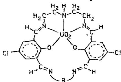
Complexes [\text{UO}_2\text{B}]
