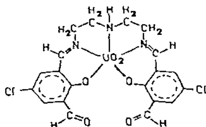
Complex [\text{UO}_2\text{A}]
