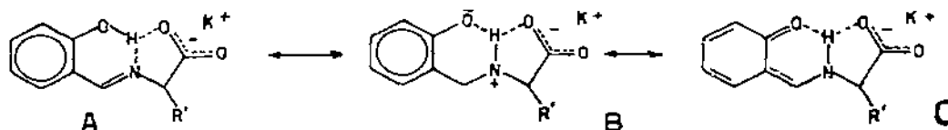
Fig. 7. The possible tautomeric forms of the salicylaldimine- \alpha -aminoacids.
