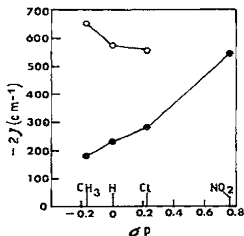
Fig. 9. The relations between the -2J values and Hammett's \sigma_p values for (\text{VO})_2\text{fsal}(\text{ap-R})_2(\text{OCH}_3) (●) and \text{Cu}_2\text{fsal}(\text{ap-R})_2(\text{OCH}_3) (○).
